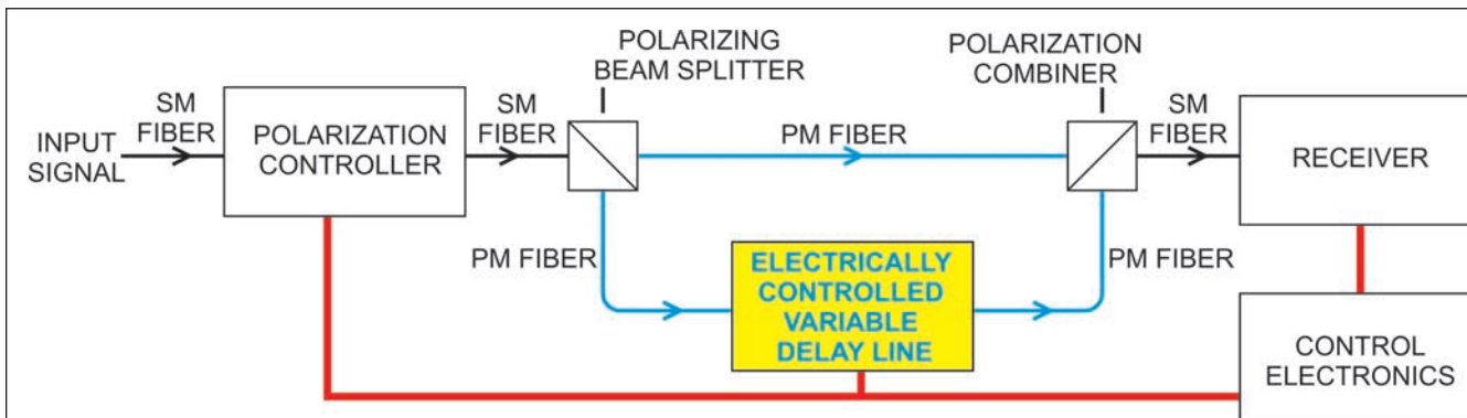
Figure 9. PMD Compensation System Using a Variable Delay Line
