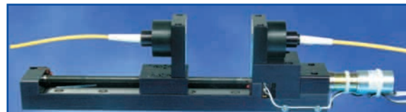
Delay Line with Servo Motor (ODL-300)
