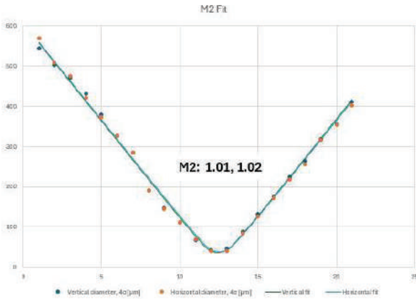
M 2 value < 1.03
